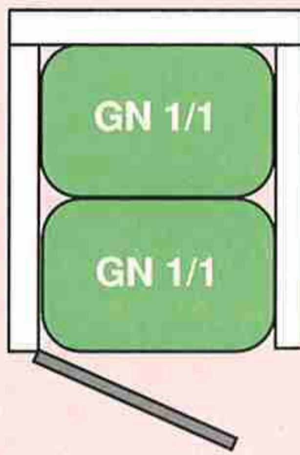
Chariot NAVIS 2/1 - 13 x 85 - 1 porte NAVIS 2/1 - 13 x 85 - 1door
